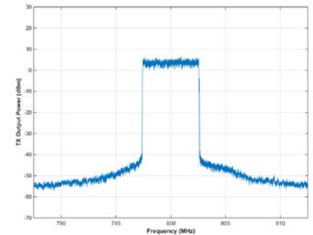
Figure 8: 5MHz 5G-NR
