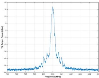
Figure 6: GMSK
